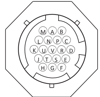
19-pin Connector
